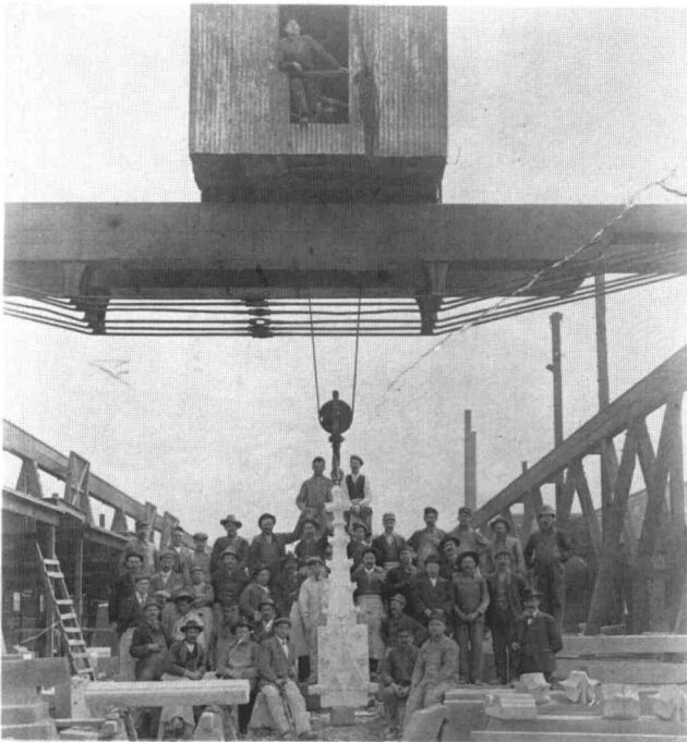
Figure 19. A traveling crane at the Swenson stonecutting sheds, photographed by the T. M. Knight View Co. of St. Louis, Missouri, c1910. Workers gather while a postcard photographer documents the completion of an ornamental crocket, probably for a church spire. Until recently, the Swensons specialized in building stone, the First Church of Christ Scientist in Boston and the Waldorf Astoria Hotel in New York being among their first major contracts. Courtesy of the New Hampshire Historical Society; gift of Judith F. Mason, F4205.
