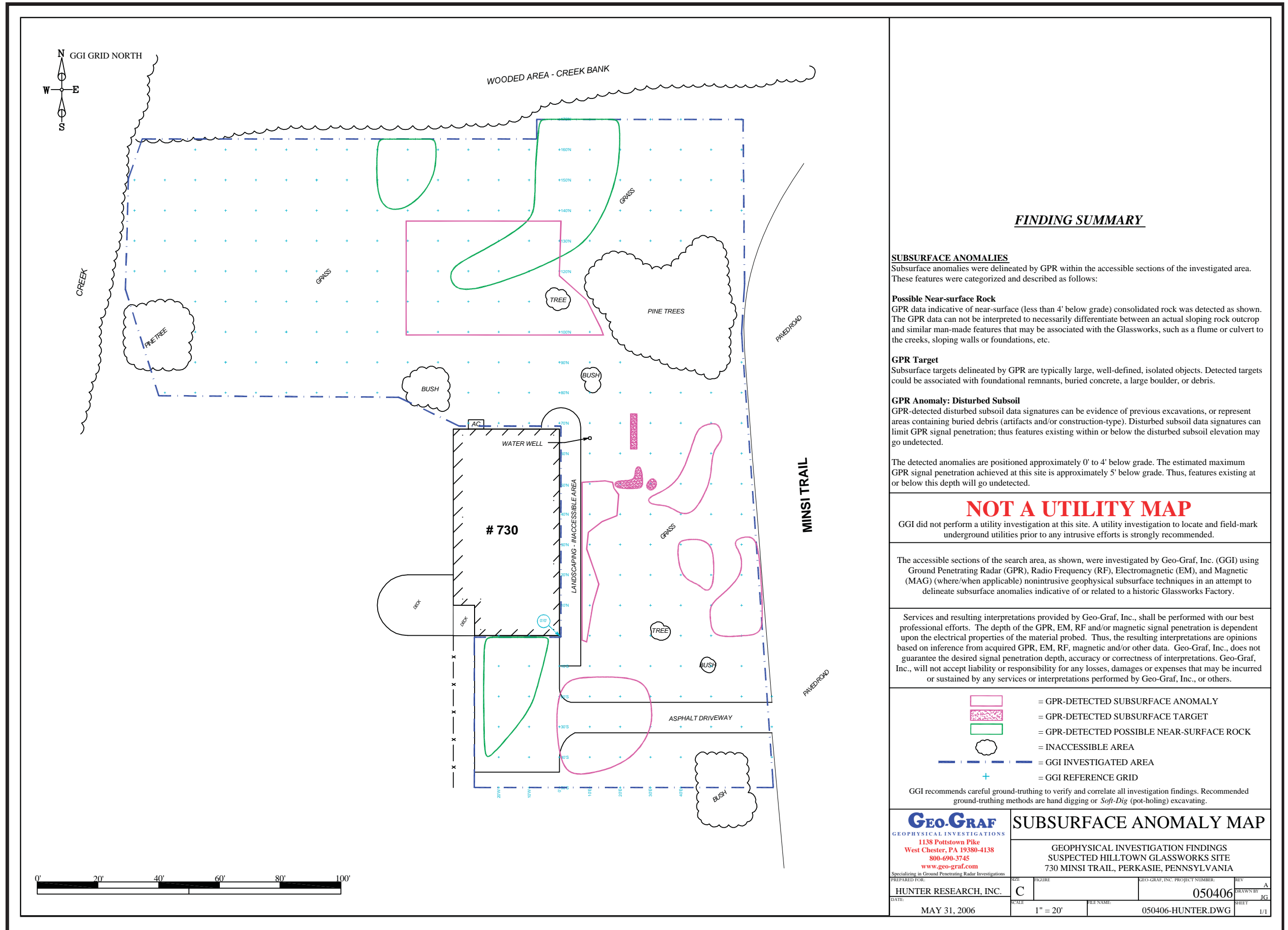
Figure 3. Hilltown Glasshouse [36Bu332]: Geophysical Map of Subsurface Anomalies.
