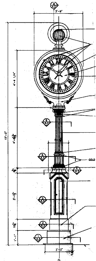
This shop drawing of the Yorkville Clock was made by Historical Arts and Casting, Inc., in preparation for the restoration of the century-old sidewalk clock. Courtesy of Margot Gayle
